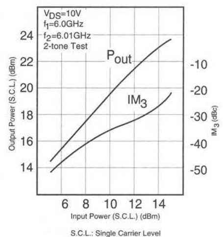
OUTPUT POWER & IM_3 vs INPUT POWER
