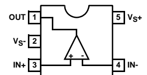
EL5191 (5-PIN SOT-23) TOP VIEW
