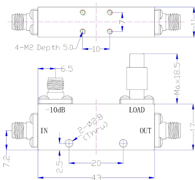
Dimensions (Unit: mm/[inch], Tolerance: ±0.5mm)
